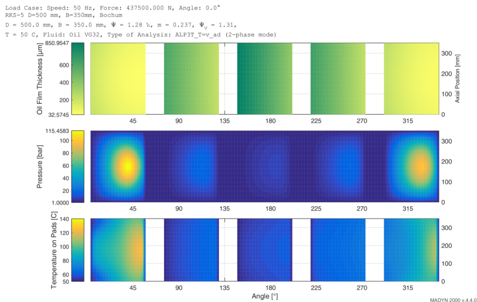
Fig. 3.8: Field plots of MADYN 2000 results for oil film thickness, pressure distribution and pad surface temperature
