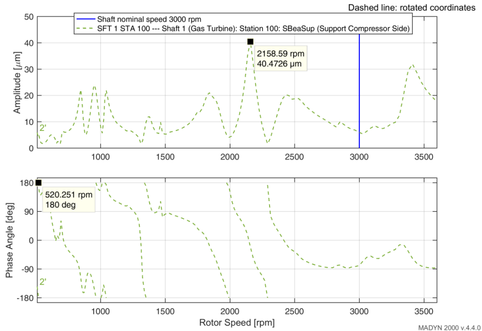
Fig. 1.22: Resonance curve of the response to identified load
