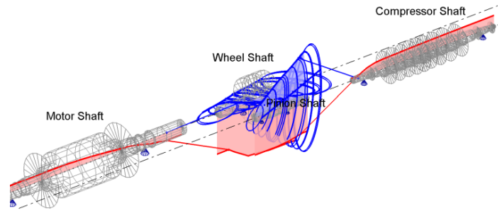
Coupled lateral torsional vibration mode
